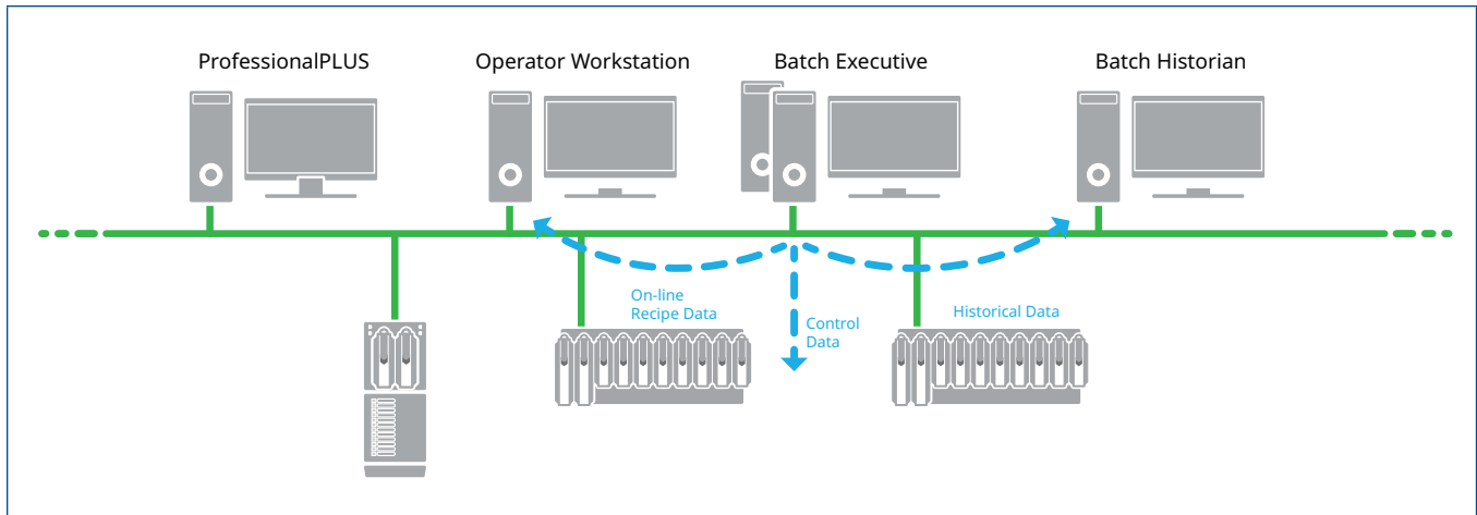
The Batch Executive processes and serves data to the DeltaV Batch application suite.
